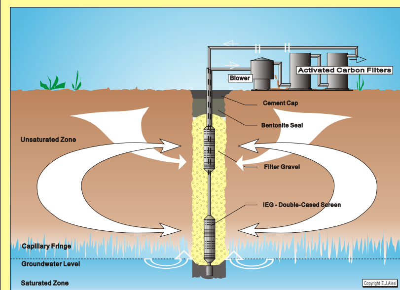
IEG Soil Air Circulation-Vacuum Vapour Extraction™ System (IEG SAC-VVE™ Process)
