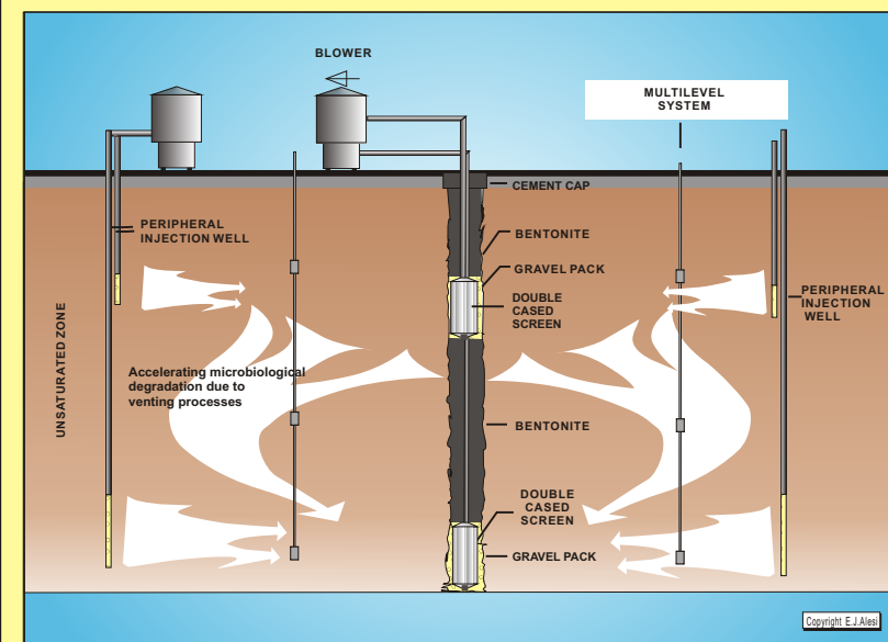
Soil Air Circulation-Bioventing™ for microbiological degradation of non-volatile contaminants (IEG SAC-Bioventing™ Process)
